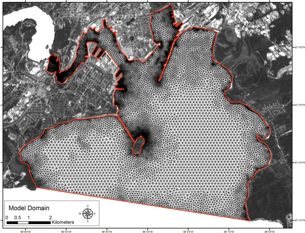
Figure 3 -- Model Mesh and Domain Overview
